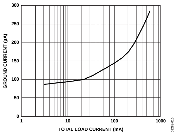
Figure 18. Ground Current vs. Load Current, All Outputs Loaded Equally, V_{RIPPLE} = 50\text{ mV} , C_{OUT} = 1\text{ }\mu\text{F}
