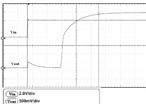
Figure 13. Enable transient
