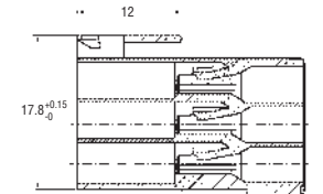
Section X-X
