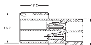
Section X-X
