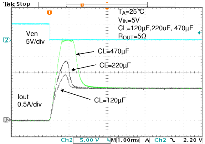
Inrush Current
