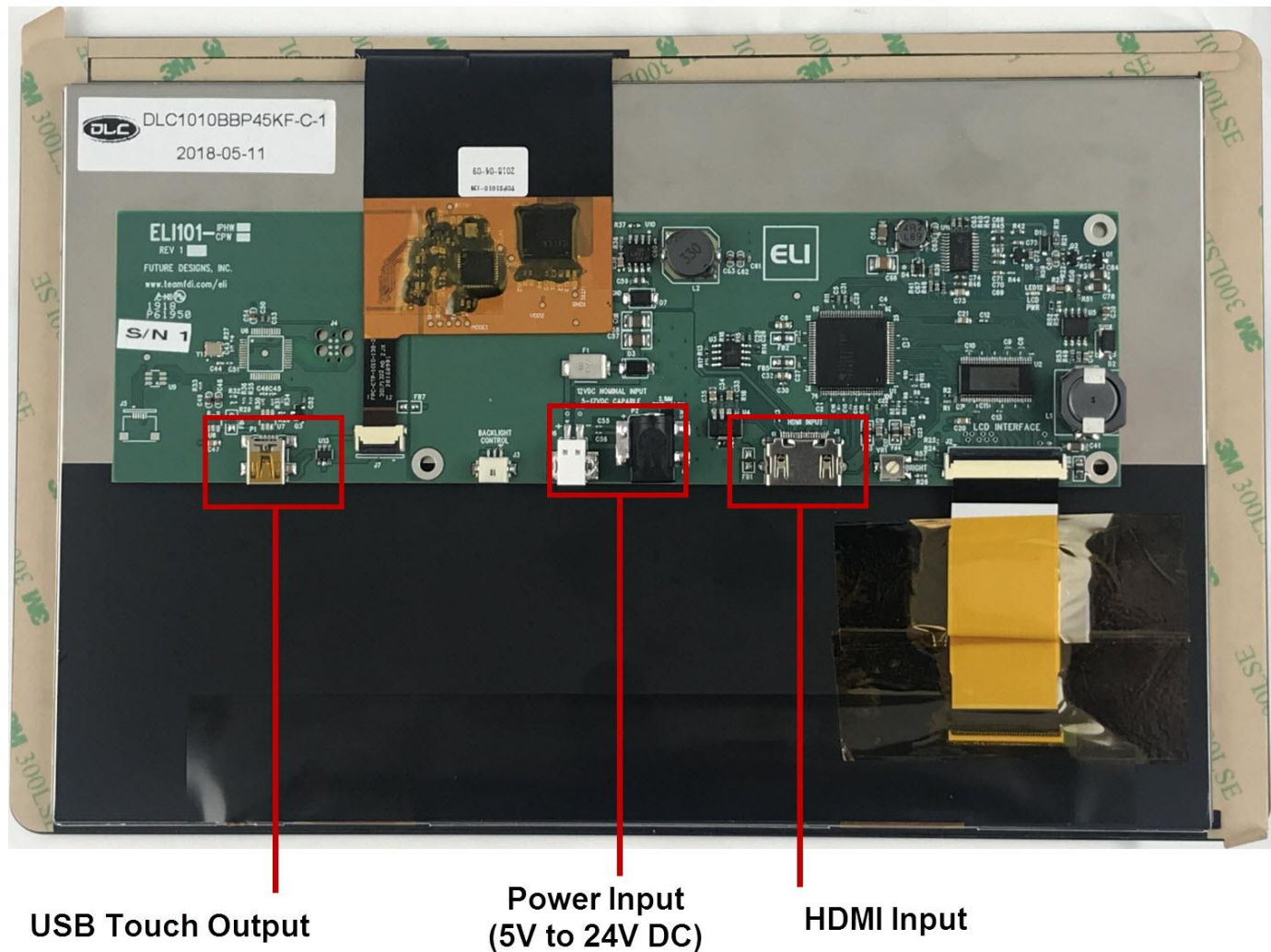
Figure 2. ELI101-IPHW Connectors
