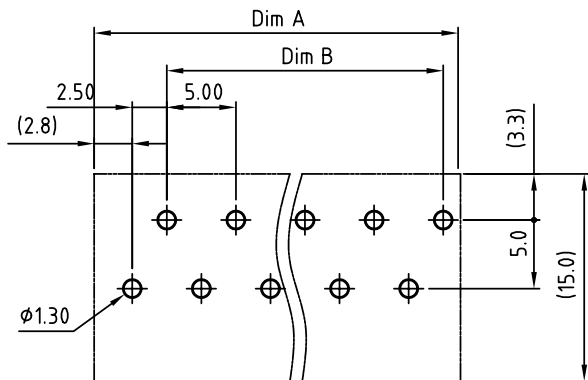
PCB Layout
