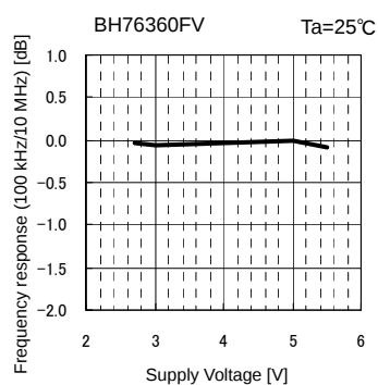
Fig.35 GF vs. Supply Voltage
