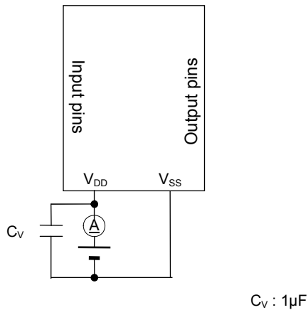
Measuring circuit 1
