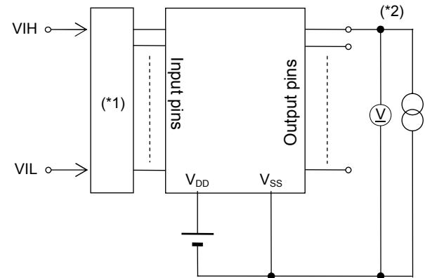
Measuring circuit 2
