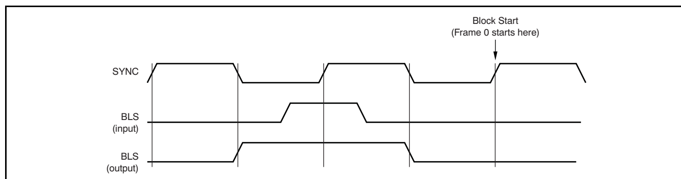
Figure 66. DIT Block Start Timing
