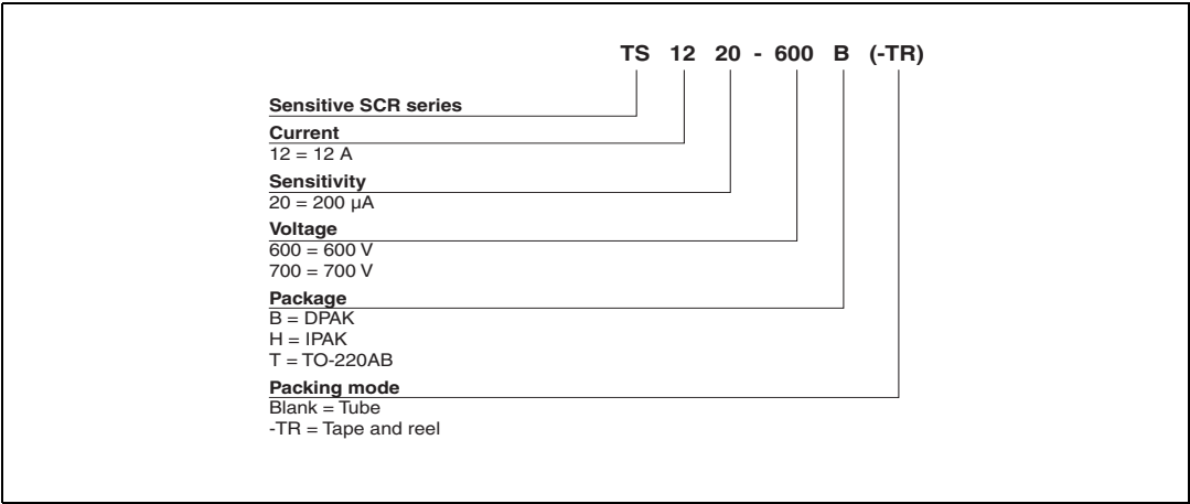
Figure 16. TS1220 series
