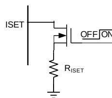
Figure 4— ISET Logic Control
