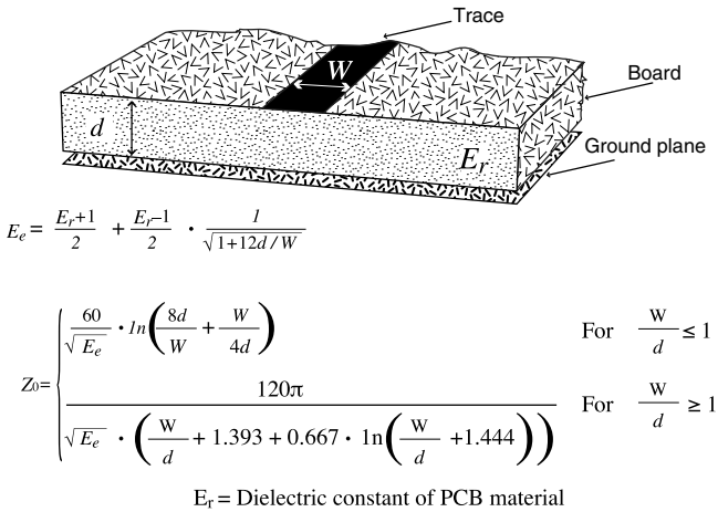
Figure 37: Microstrip Formulas
