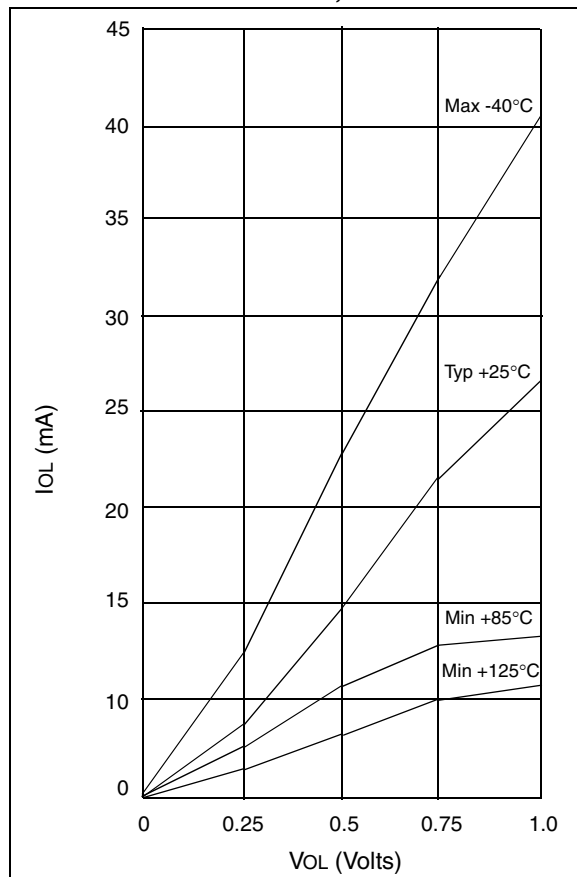
FIGURE 13-8: I_{OL} vs. V_{OL} , V_{DD} = 3.5 V
