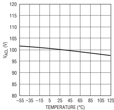
Analog Current Limit Voltage V ACL vs Temperature
