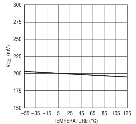
Fast Current Limit Voltage V FCL vs Temperature
