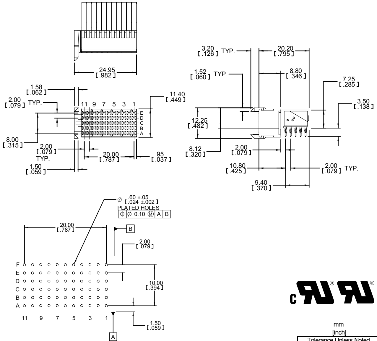
Recommended PCB hole mounting pattern Connector side
