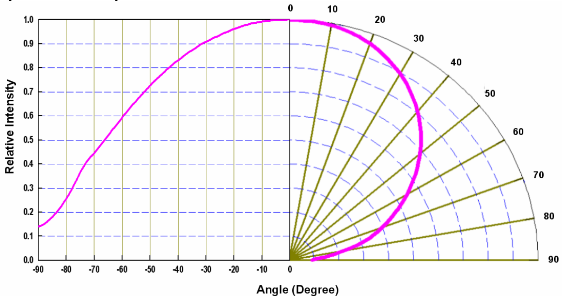
Typical Representative Spatial Radiation Pattern
