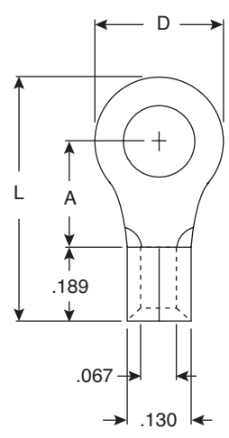
Dimensions: In.
