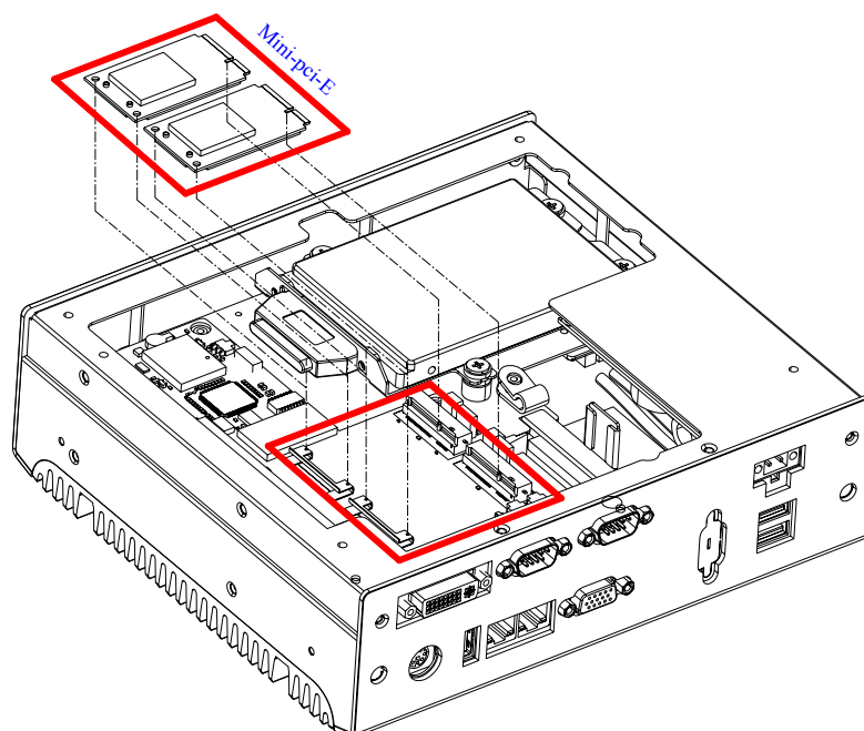
Figure 2.9 MiniPCIe Add-on card installation
