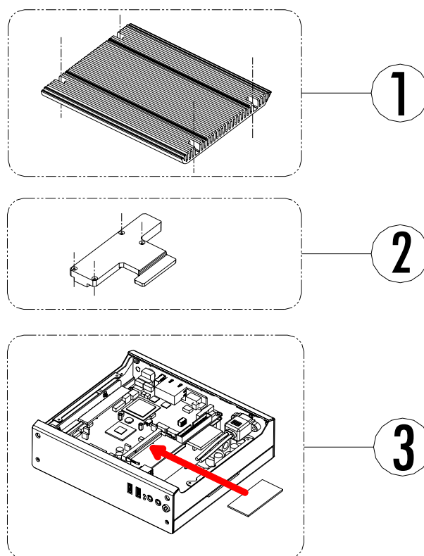
Figure 2.6 Memory Installation
