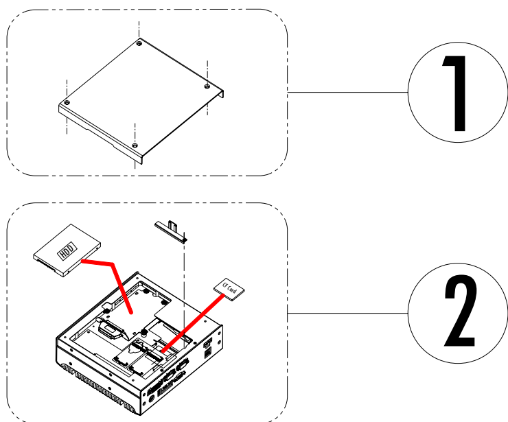
Figure 2.8 Internal Fixed HDD Installation
