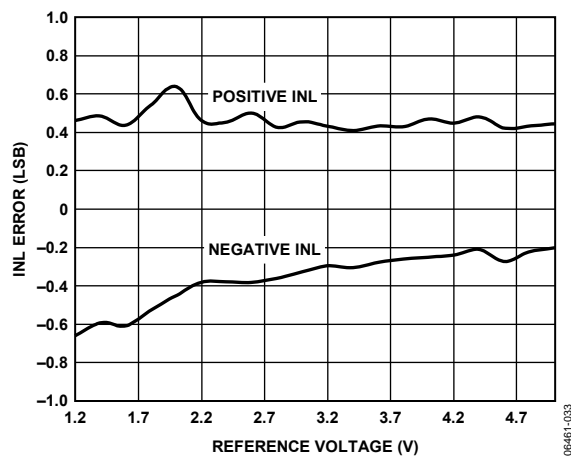
Figure 7. INL Error vs. Reference Voltage, f_{SCL} = 1.7\text{ MHz} Without Clock Stretching
