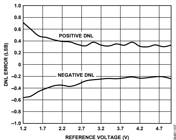
Figure 8. DNL Error vs. Reference Voltage, f_{SCL} = 1.7\text{ MHz} Without Clock Stretching
