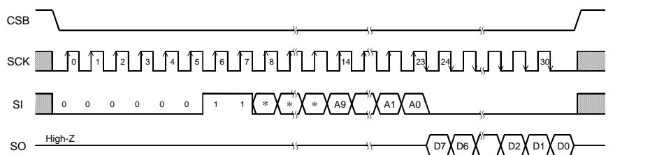
Figure 37. Read command
