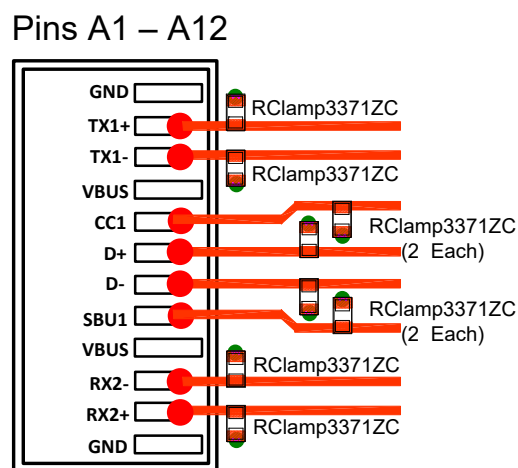
Figure 1 - USB Type-C Top Layer Protection Example
