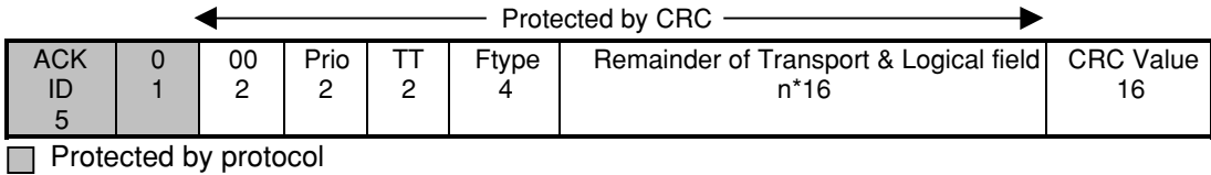
Figure 11. CRC Checking
