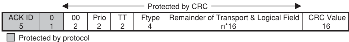
Figure 2. TX CRC Generator
