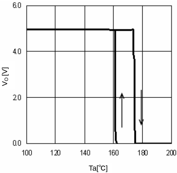
Fig.28 TSD ( I_o=0mA )
