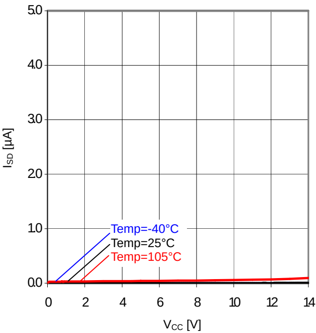
Fig.26 V_{CC} - I_{SD} ( V_{EN}=0\text{V} )
