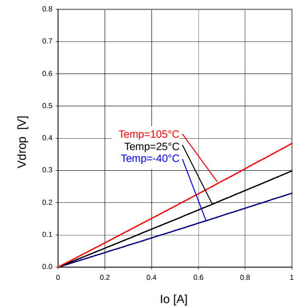
Fig.37 Minimum dropout Voltage 4 (V CC =10.0V)
