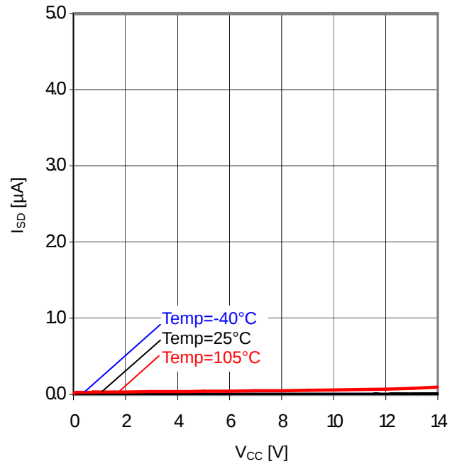
Fig.26 V_{CC} - I_{SD} ( V_{EN}=0\text{V} )
