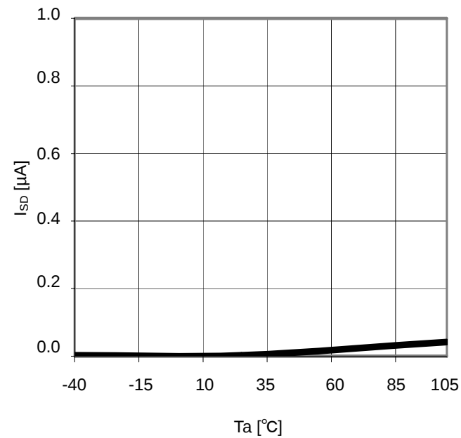
Fig.23 T_a - I_{SD} ( V_{EN}=0\text{V} )
