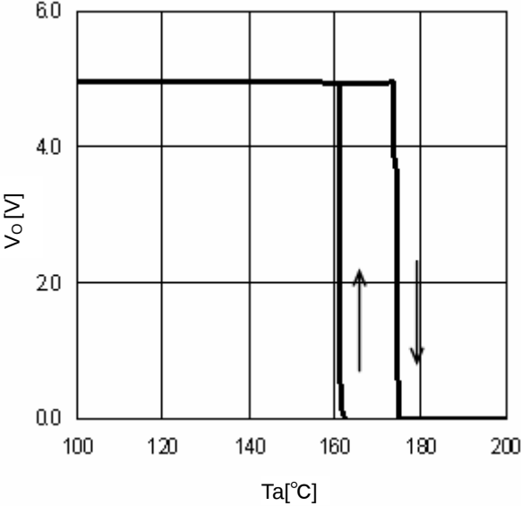
Fig.28 TSD ( I_O=0mA )
