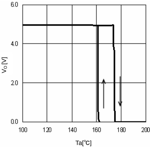
Fig.28 TSD ( I_o=0mA )
