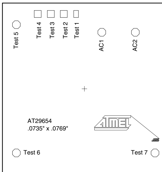
Figure 3. Die Layout
