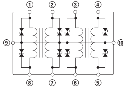
①~⑥: Data Line; ⑨ and ⑩:Ground
