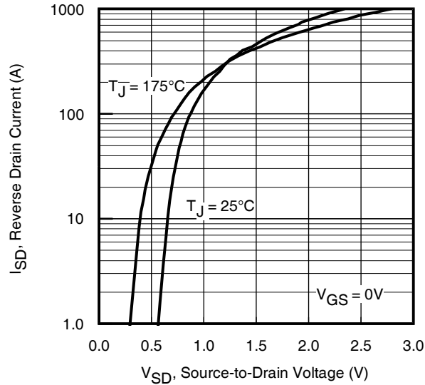
Fig 10. Typical Source-Drain Diode Forward Voltage
