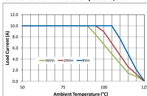
Load Current vs. Ambient Temperature, 200 LFM
