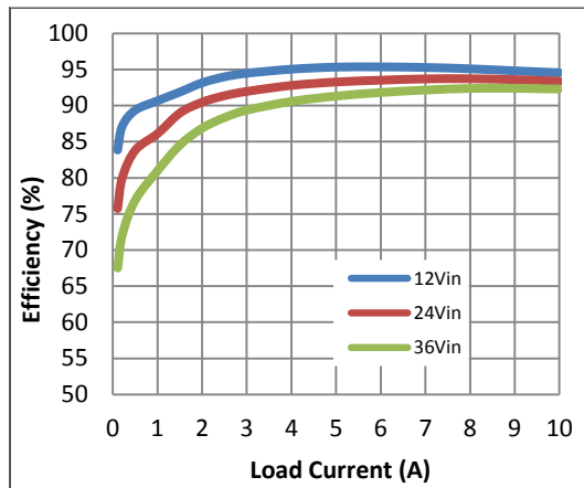
Efficiency at 25°C
