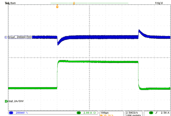
Transient Response: 2A to 7A, at 5A/μs
