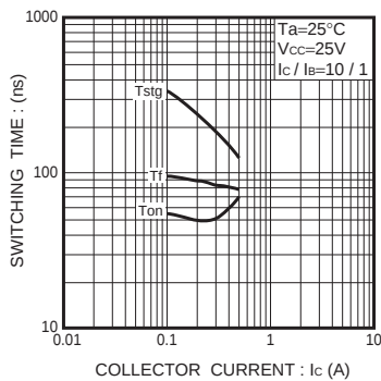
Fig.1 Switching Time
