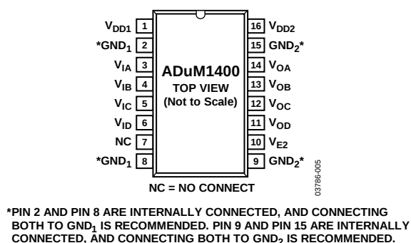
Figure 5. ADuM1400 Pin Configuration
