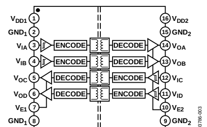
Figure 3. ADuM1402
