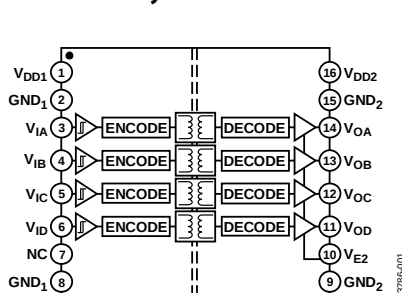
Figure 1. ADuM1400
