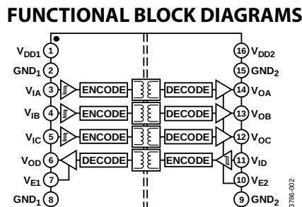
Figure 2. ADuM1401
