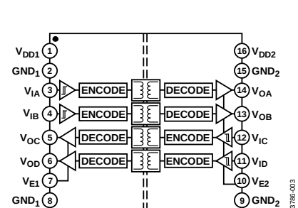
Figure 3. ADuM1402
