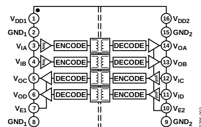
Figure 3. ADuM1402
