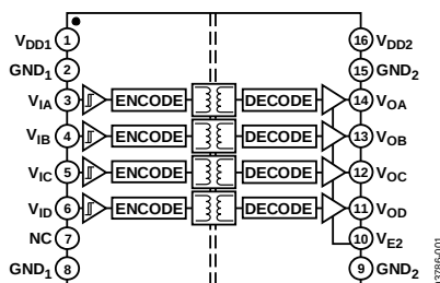
Figure 1. ADuM1400
