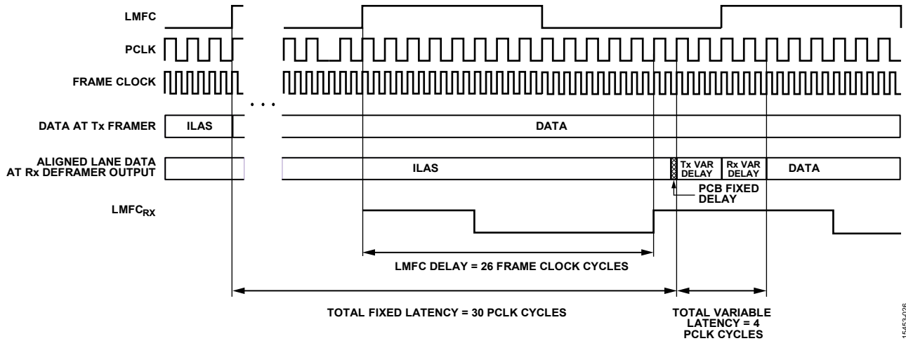
Figure 60. LMFC Delay Calculation Example
