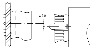
Allowed misalignment
