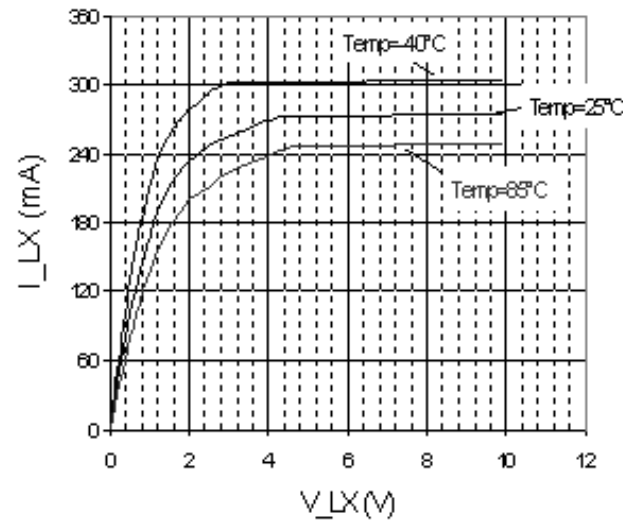
Figure 15. Low Side ON-Resistance Temperature Characteristics
