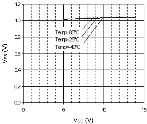
Figure 11. FB Threshold Voltage vs V_{CC}
