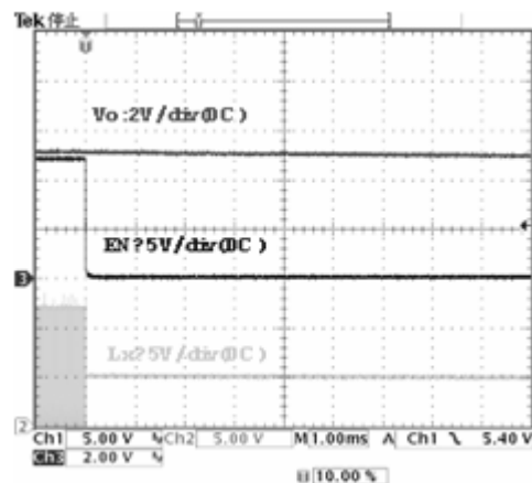
Figure 25. Stop Waveform
