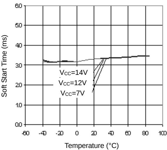
Figure 13. Soft Start Time vs Temperature
