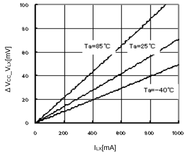
Figure 14. High Side FET ON-Resistance Temperature Characteristics
