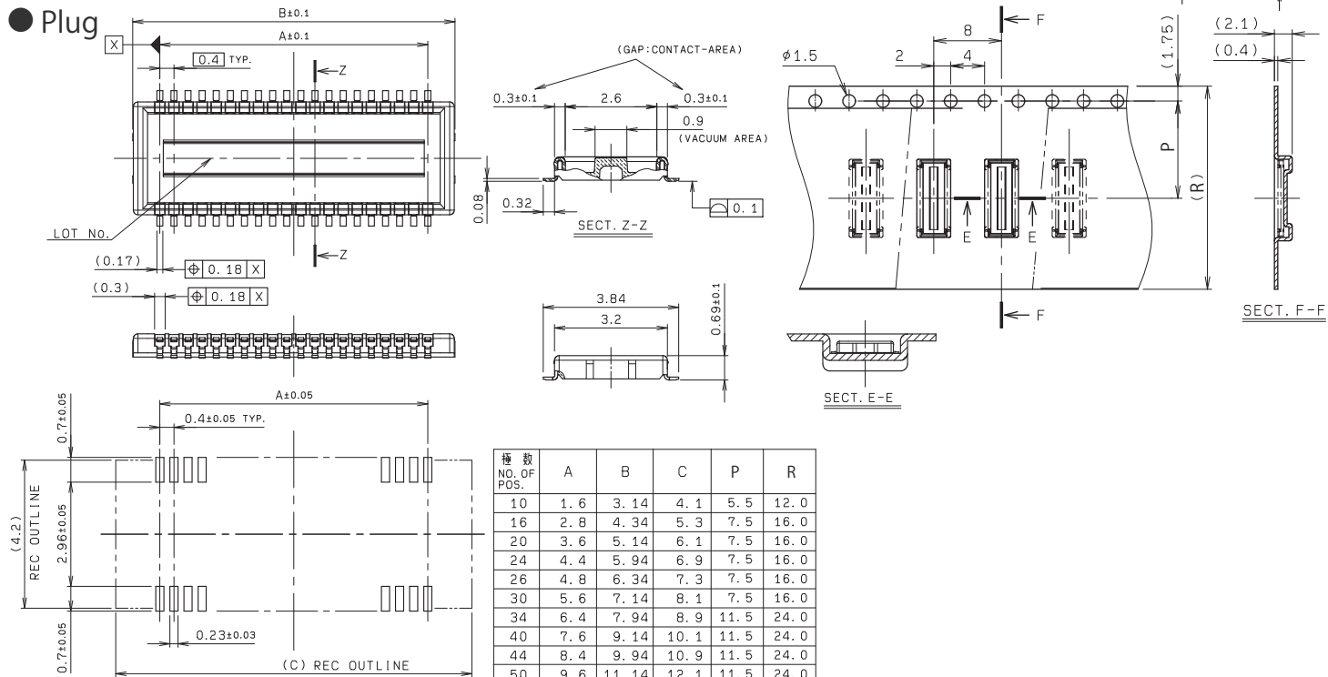
MOUNTING LAYOUT
