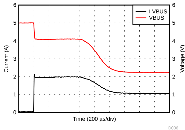
Figure 24. PP_5V0 Current Limit with a Soft Short (2 Ω)
