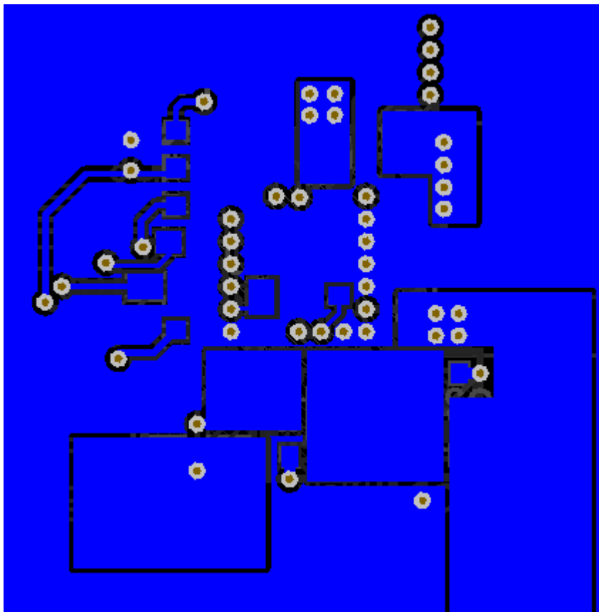
Figure 105. Final Routing (Bottom Layer)
