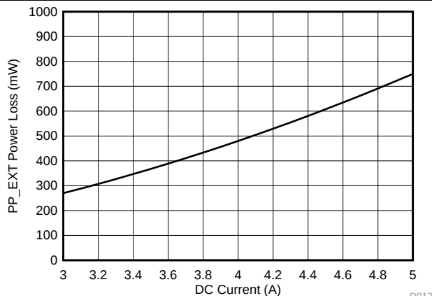
Figure 78. PP_EXT Power Loss
