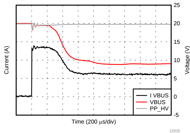
Figure 28. PP_HV Current Limit Response with a Soft Short (7 \Omega )
