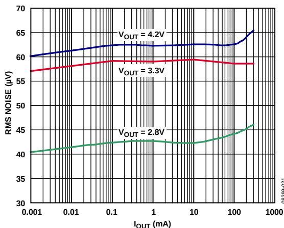
Figure 25. Output Noise vs. Load Current and Output Voltage
