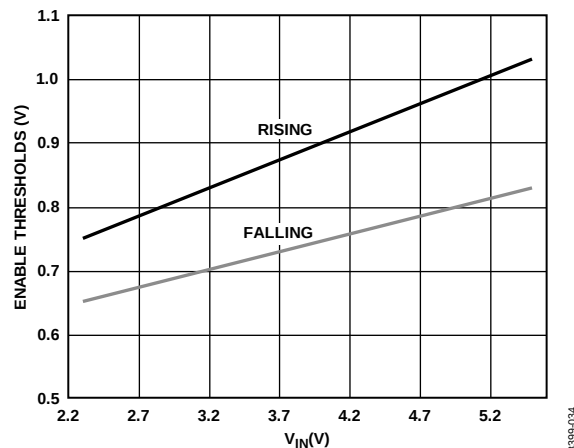
Figure 36. Typical EN Pin Thresholds vs. Input Voltage
