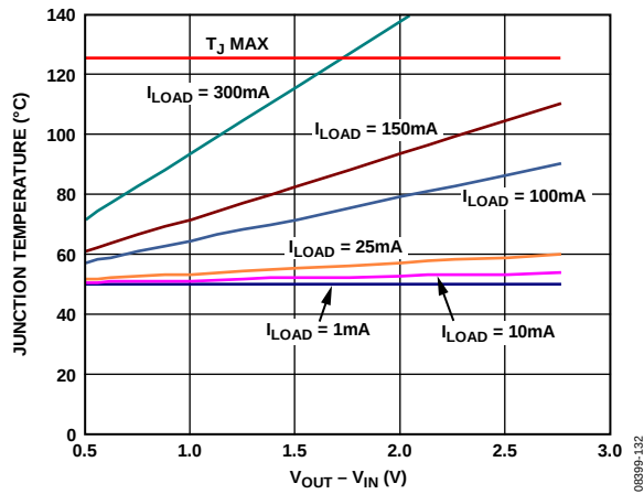
Figure 42. Junction Temperature vs. Power Dissipation, 100 mm 2 of PCB Copper, T_A = 50^\circ\text{C}
