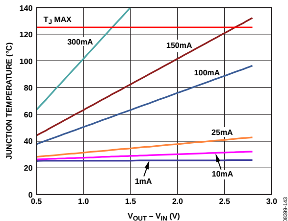
Figure 49. Junction Temperature vs. Power Dissipation, 0 mm 2 of PCB Copper, T_A = 25^\circ\text{C}
