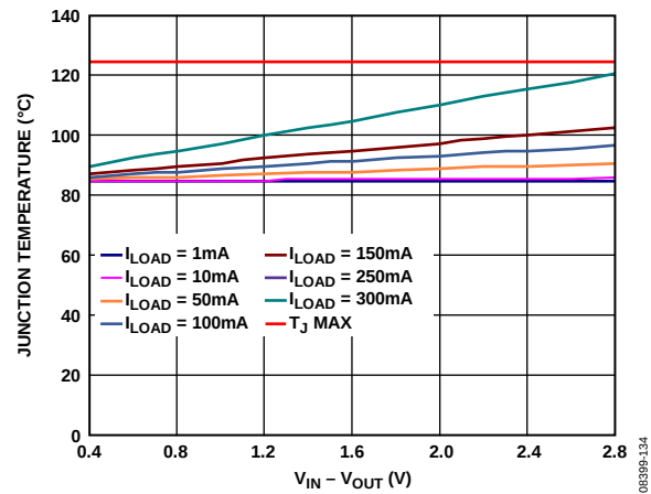
Figure 44. Junction Temperature vs. Power Dissipation, Board Temperature = 85^\circ\text{C}
