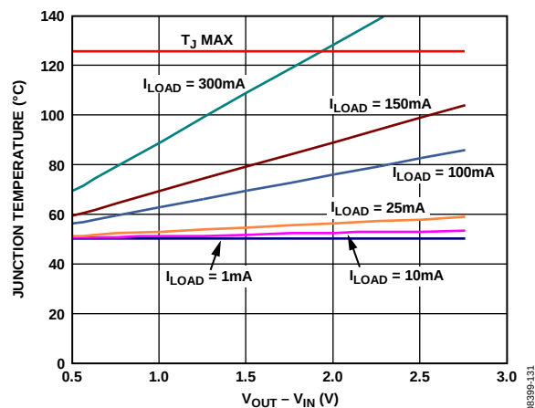
Figure 41. Junction Temperature vs. Power Dissipation, 500 mm 2 of PCB Copper, T_A = 50^\circ\text{C}
