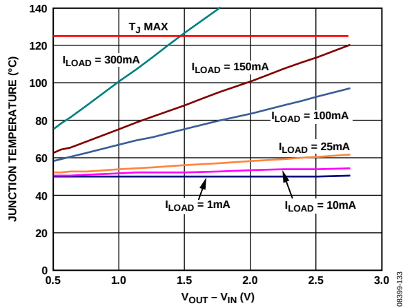
Figure 43. Junction Temperature vs. Power Dissipation, 0 mm 2 of PCB Copper, T_A = 50^\circ\text{C}
