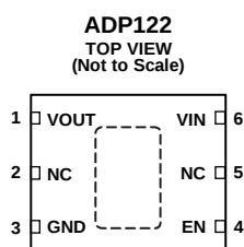
Figure 5. ADP122 TSOT Fixed Output Pin Configuration
