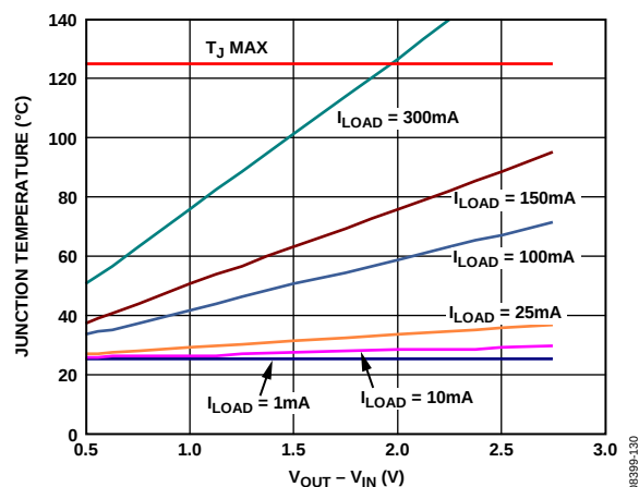
Figure 40. Junction Temperature vs. Power Dissipation, 0 mm 2 of PCB Copper, T_A = 25^\circ\text{C}
