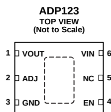
Figure 7. ADP123 TSOT Adjustable Output Pin Configuration
