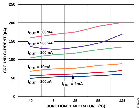
Figure 12. Ground Current vs. Junction Temperature
