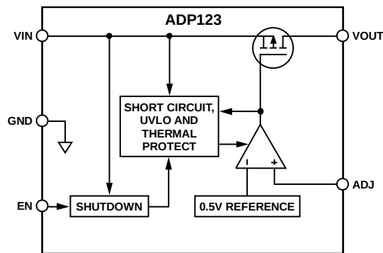
Figure 31. ADP123 Internal Block Diagram (Adjustable Output)
