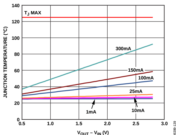
Figure 45. Junction Temperature vs. Power Dissipation, 500 mm 2 of PCB Copper, T_A = 25^\circ\text{C}
