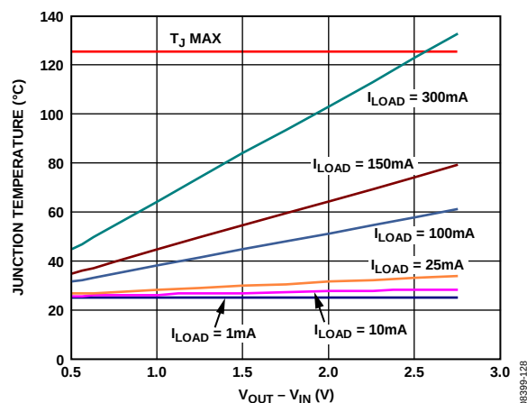
Figure 38. Junction Temperature vs. Power Dissipation, 500 mm 2 of PCB Copper, T_A = 25^\circ\text{C}
