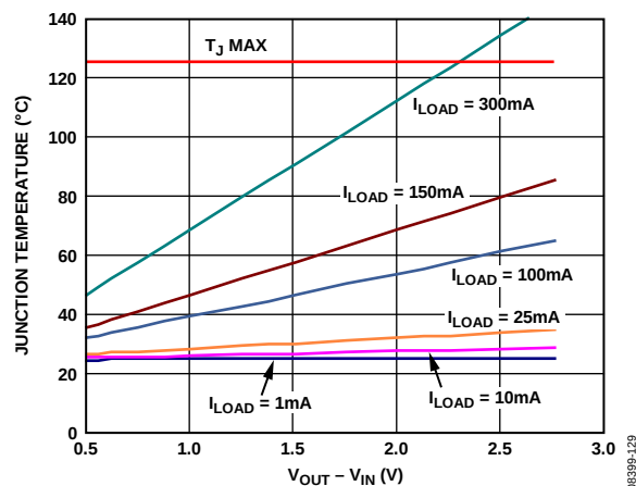
Figure 39. Junction Temperature vs. Power Dissipation, 100 mm 2 of PCB Copper, T_A = 25^\circ\text{C}
