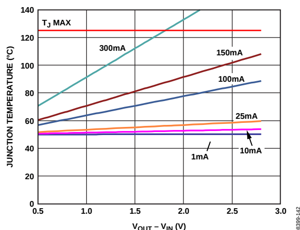
Figure 48. Junction Temperature vs. Power Dissipation, 100 mm 2 of PCB Copper, T_A = 50^\circ\text{C}
