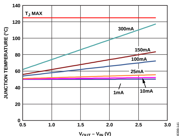
Figure 47. Junction Temperature vs. Power Dissipation, 500 mm 2 of PCB Copper, T_A = 50^\circ\text{C}
