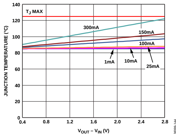
Figure 51. Junction Temperature vs. Power Dissipation, Board Temperature = 85^\circ\text{C}
