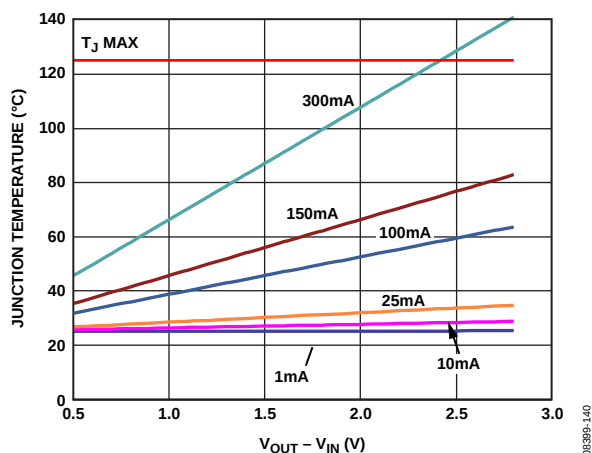
Figure 46. Junction Temperature vs. Power Dissipation, 100 mm 2 of PCB Copper, T_A = 25^\circ\text{C}
