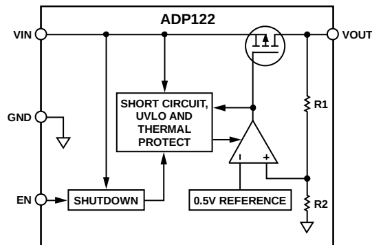
Figure 30. ADP122 Internal Block Diagram (Fixed Output)
