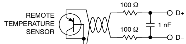
Figure 21. Filter between Remote Sensor and NCT72 Factors Affecting Diode Accuracy
