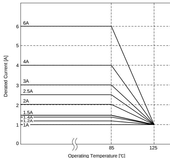
Derating
