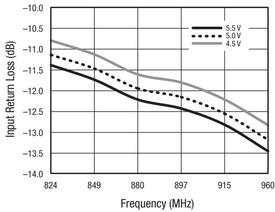
Figure 38. Input Return Loss vs Frequency Over VCC
