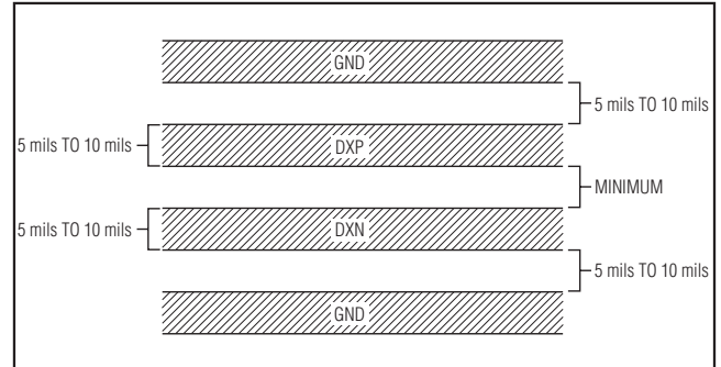
Figure 5. Recommended DXP-DXN PCB Traces. The two outer guard traces are recommended if high-voltage traces are near the DXN and DXP traces.
