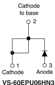
TO-247AC modified
