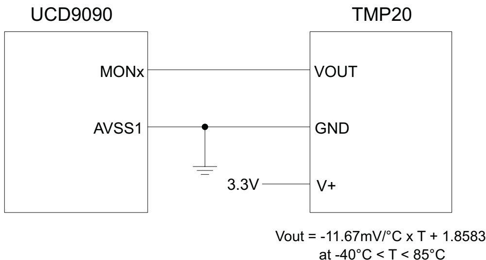
Figure 12. Remote Temperature Monitoring Circuit Example using the TMP20
