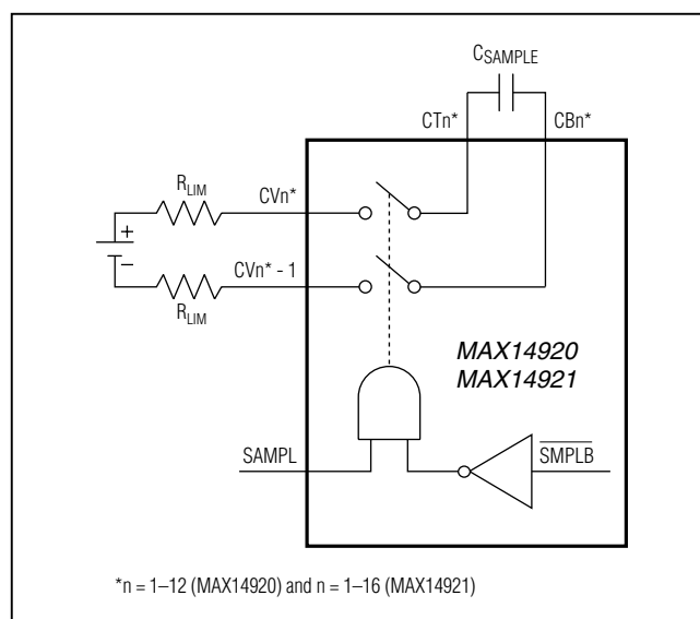
Figure 4. Voltage Sampling
