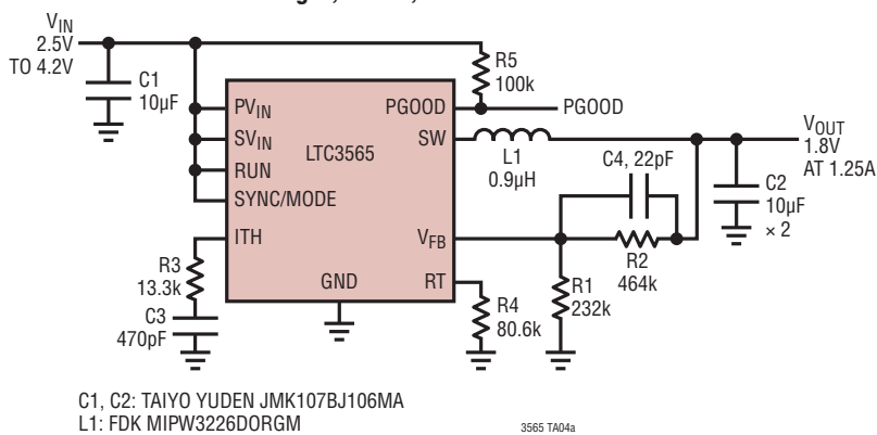
1mm Height, 2MHz, Li-Ion to 1.8V Converter
