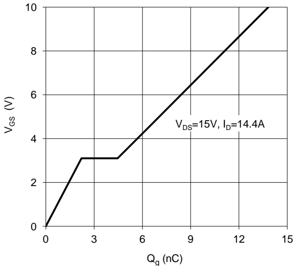
Figure 23. Gate Charge
